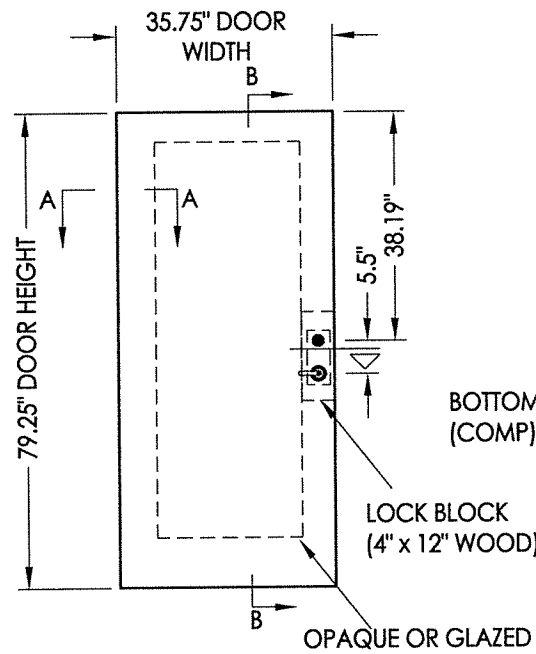
STEEL DOOR PANEL Masonite 6' 8" (Wood Edge)
